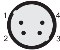
XLR-4M
